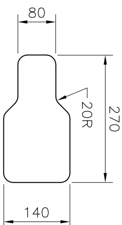
Seat (1 Off)
