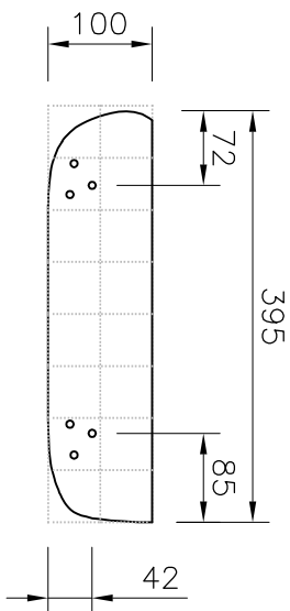
Body (2 Off) 50mm Grid
